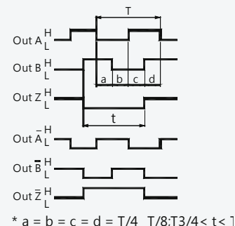
Line driver
